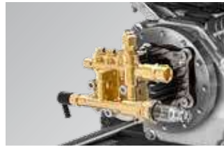
Axial pump with stainless steel pistons, brass head, double water seal
